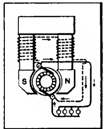
Fig. 12—Representation of a shunt-wound generator
